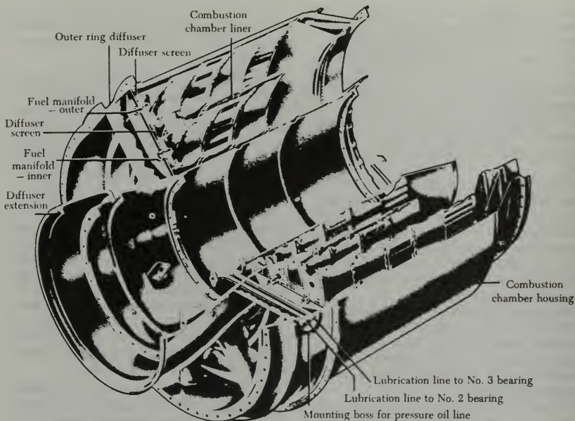
FIGURE 1-47. Double-annular combustion chamber.
